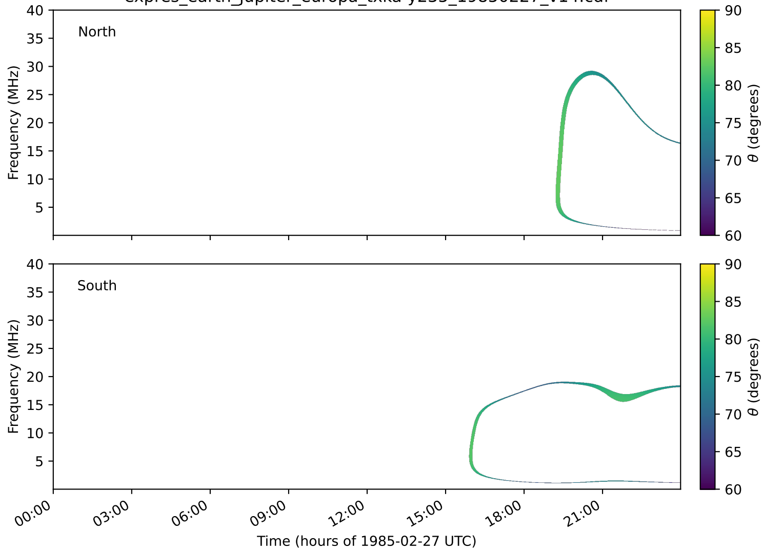
expres_earth_jupiter_europa_txka-y235_19850227_v14.cdf
