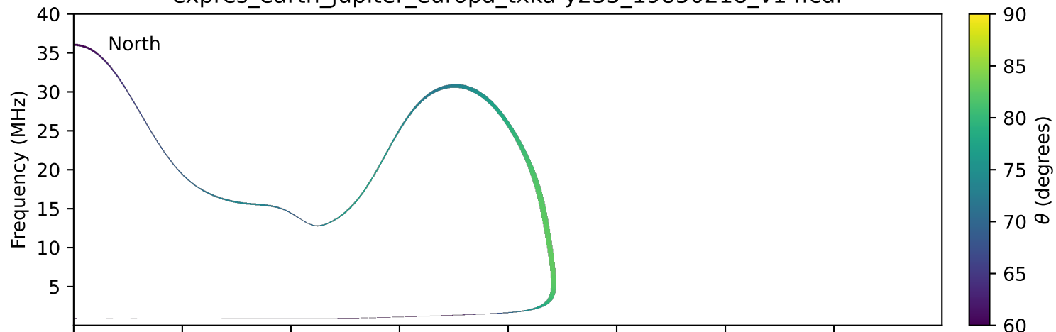
expres_earth_jupiter_europa_txka-y235_19850218_v14.cdf
