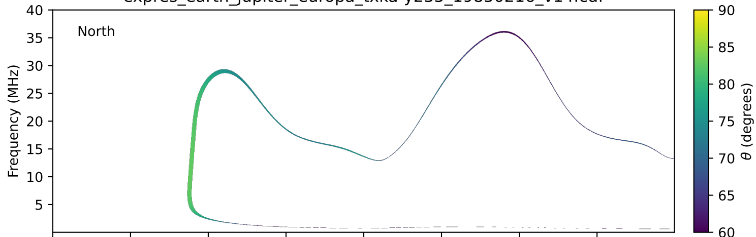
expres_earth_jupiter_europa_txka-y235_19850216_v14.cdf
