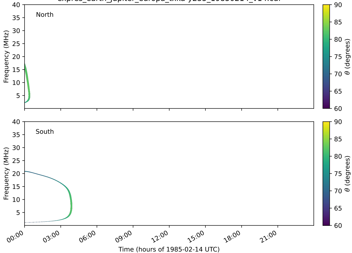
expres_earth_jupiter_europa_txka-y235_19850214_v14.cdf
