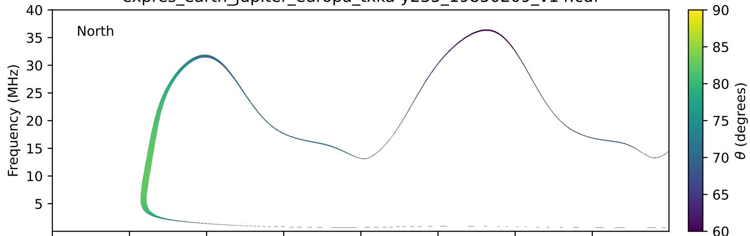
expres_earth_jupiter_europa_txka-y235_19850209_v14.cdf
