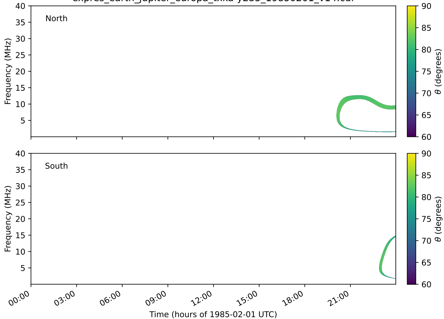
expres_earth_jupiter_europa_txka-y235_19850201_v14.cdf
