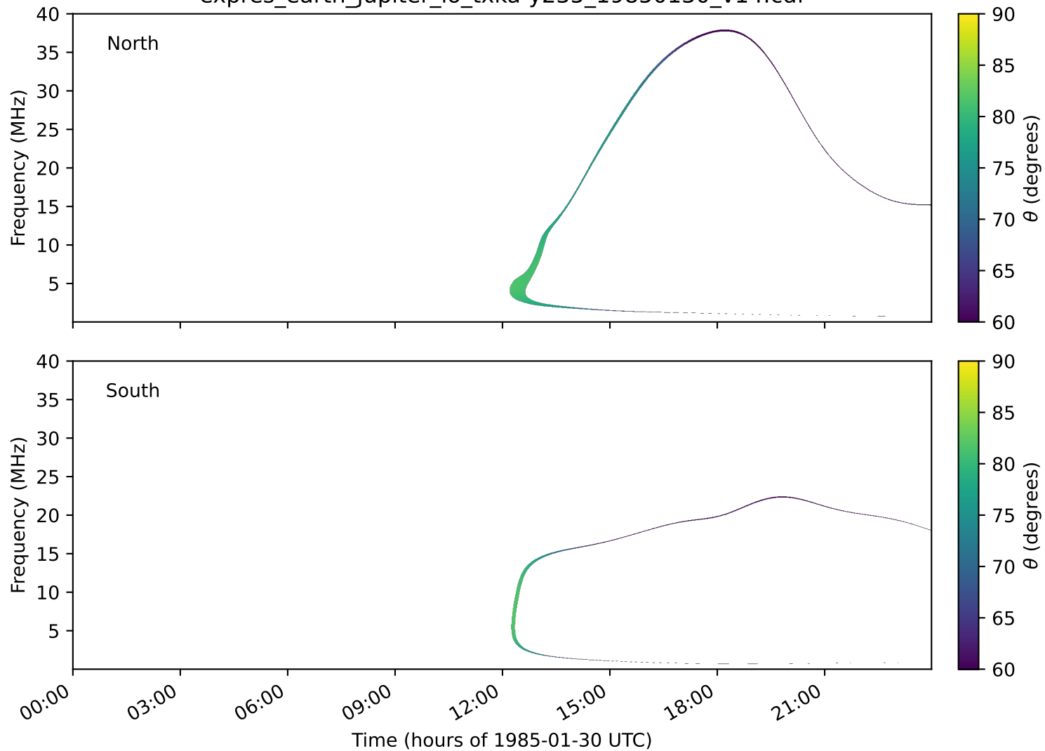
expres_earth_jupiter_io_txka-y235_19850130_v14.cdf
