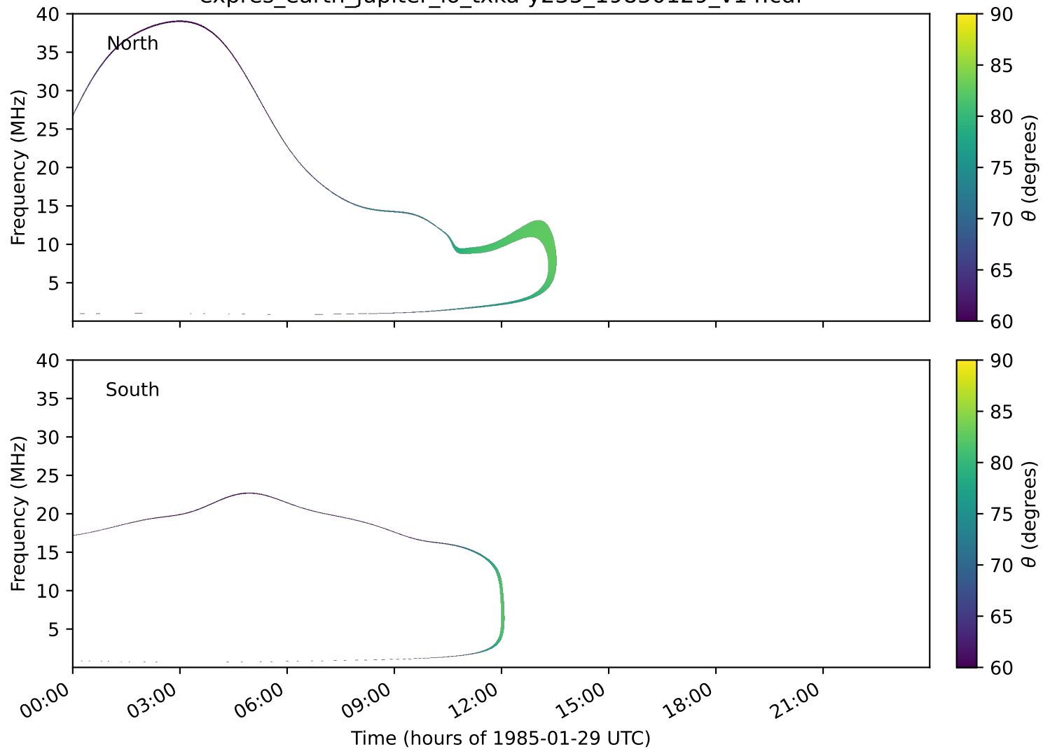
expres_earth_jupiter_io_txka-y235_19850129_v14.cdf
