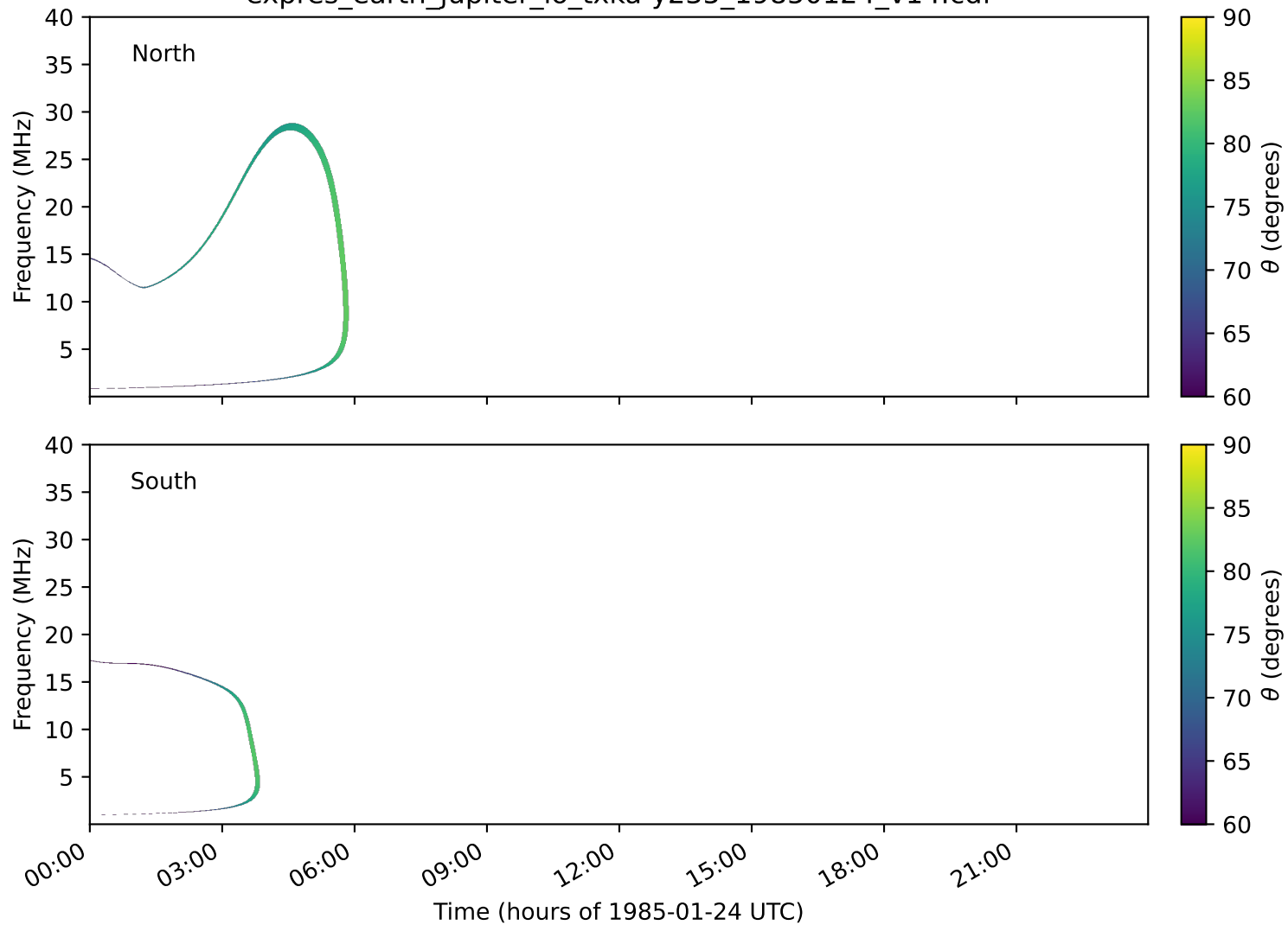
expres_earth_jupiter_io_txka-y235_19850124_v14.cdf
