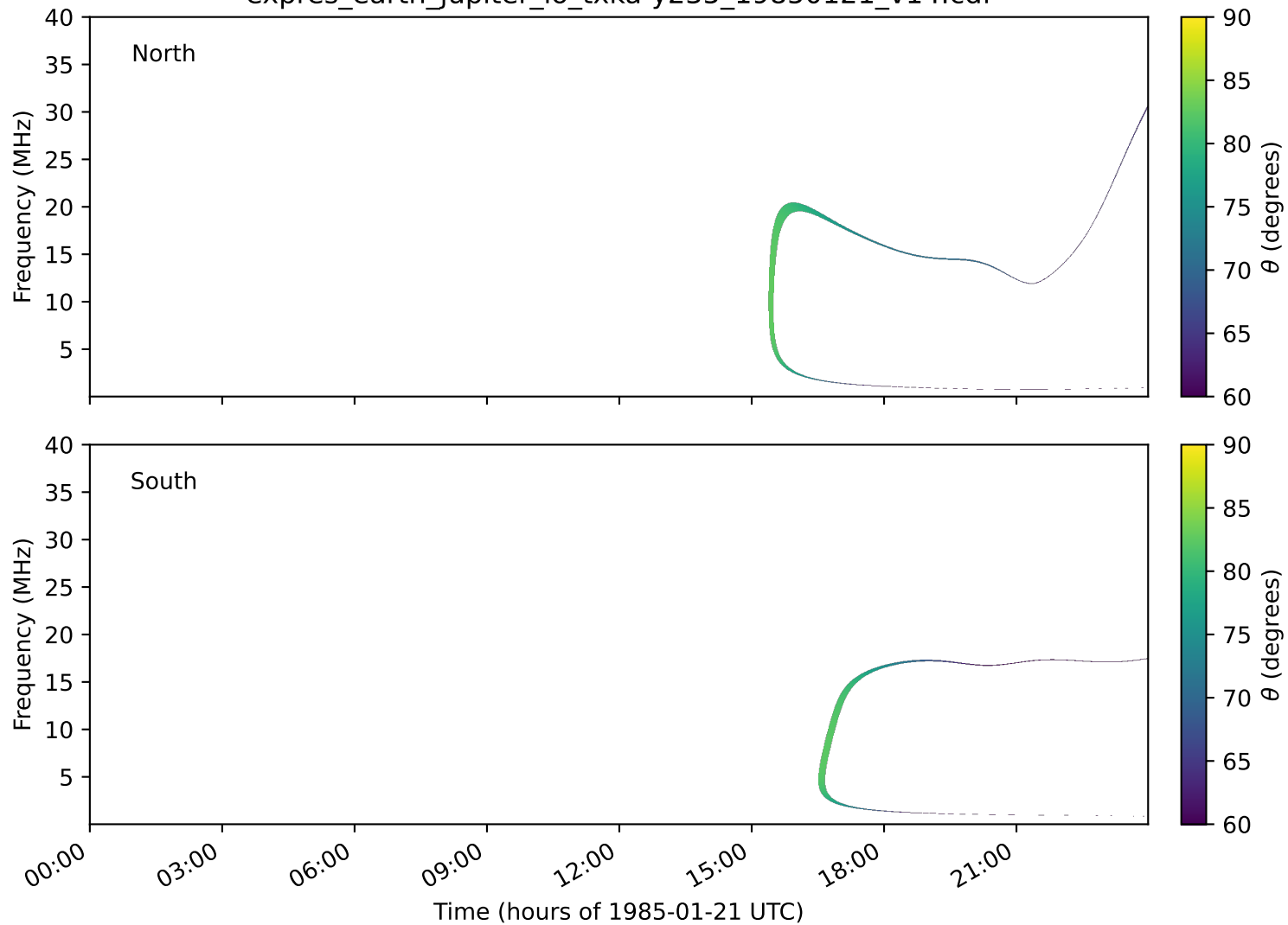
expres_earth_jupiter_io_txka-y235_19850121_v14.cdf
