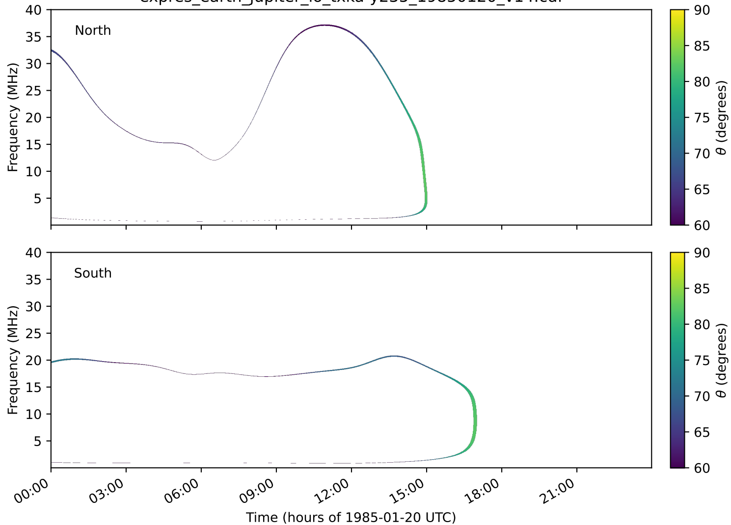
expres_earth_jupiter_io_txka-y235_19850120_v14.cdf
