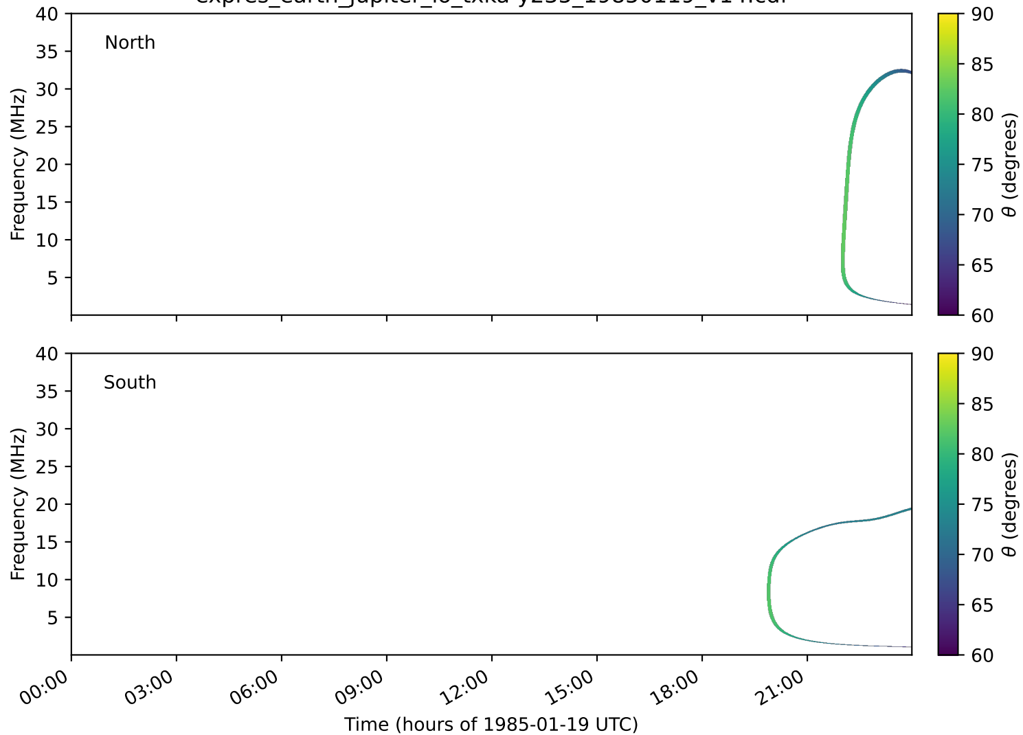
expres_earth_jupiter_io_txka-y235_19850119_v14.cdf
