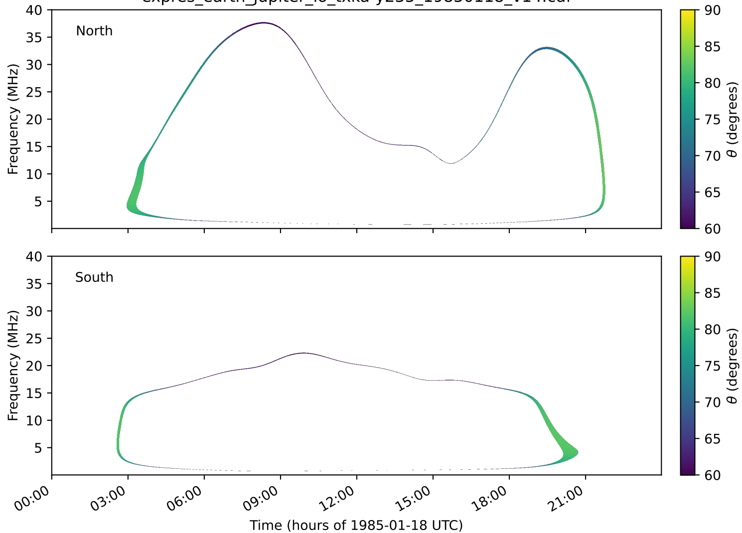
expres_earth_jupiter_io_txka-y235_19850118_v14.cdf
