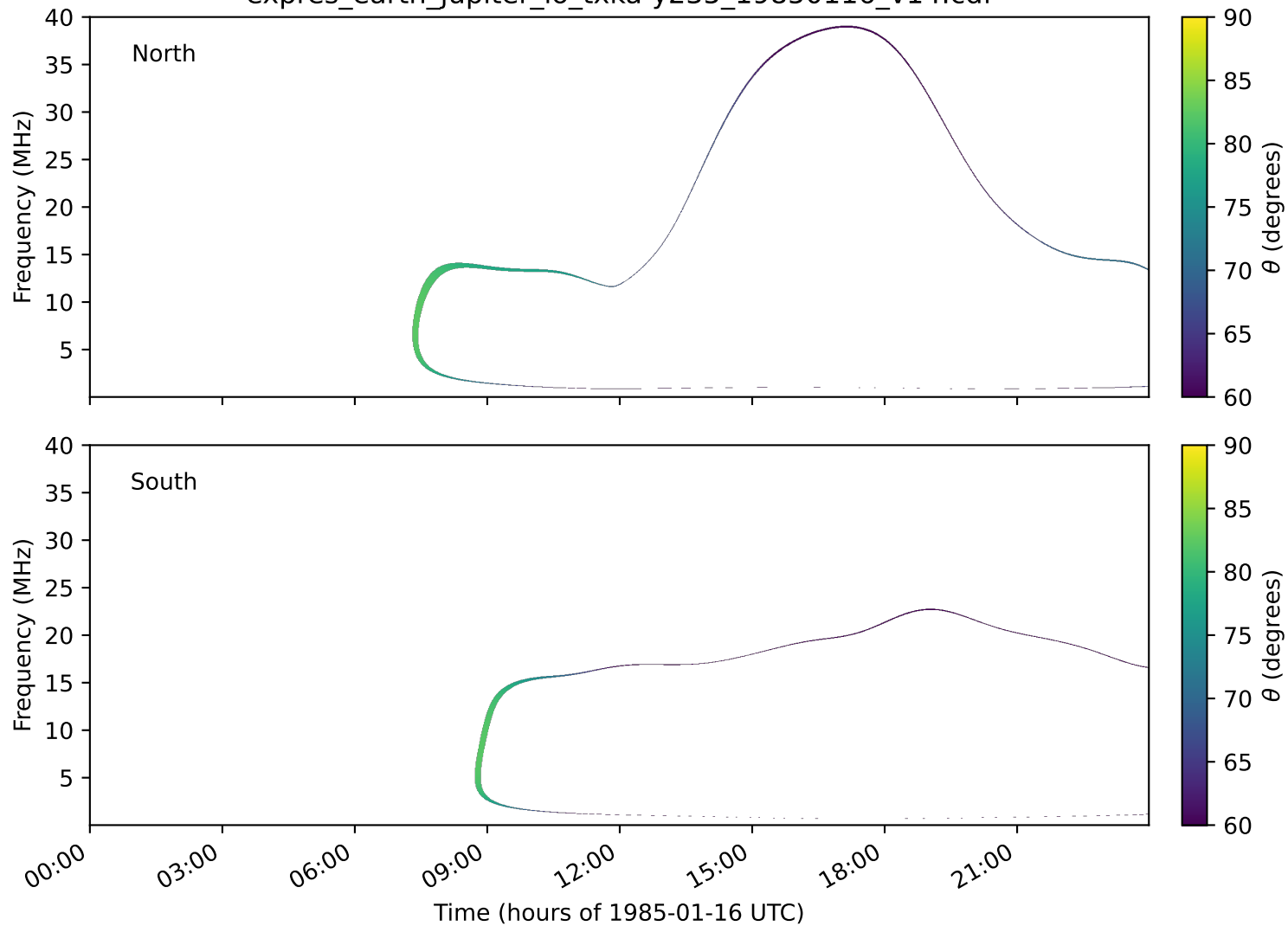
expres_earth_jupiter_io_txka-y235_19850116_v14.cdf
