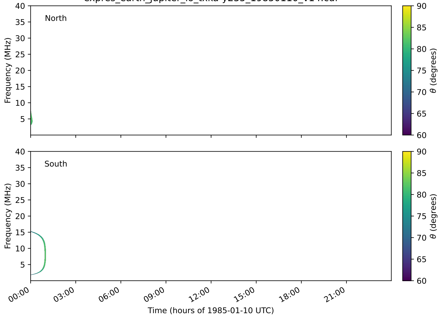
expres_earth_jupiter_io_txka-y235_19850110_v14.cdf
