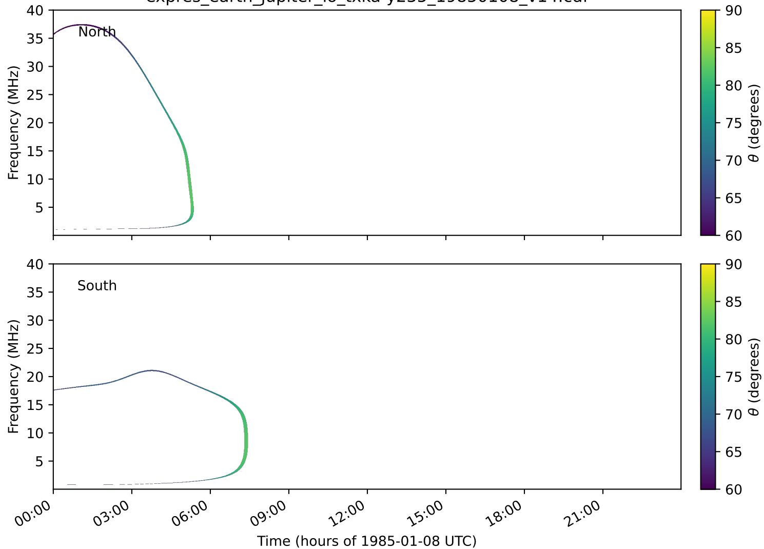
expres_earth_jupiter_io_txka-y235_19850108_v14.cdf
