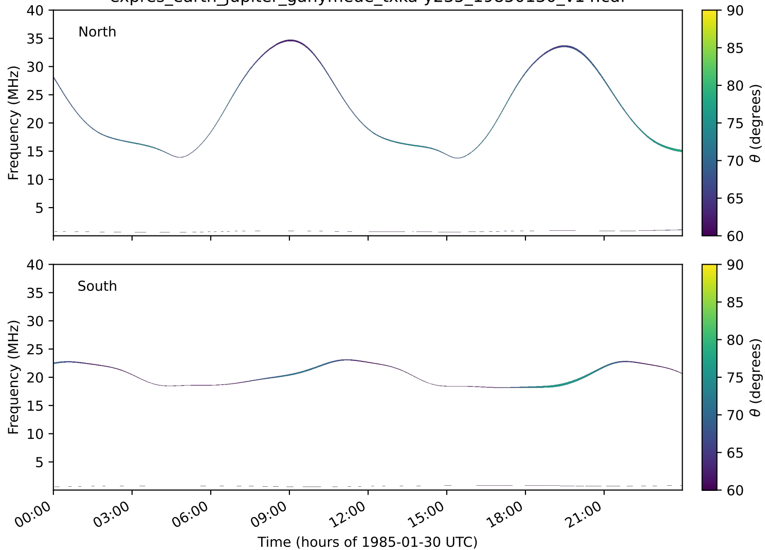
expres_earth_jupiter_ganymede_txka-y235_19850130_v14.cdf
