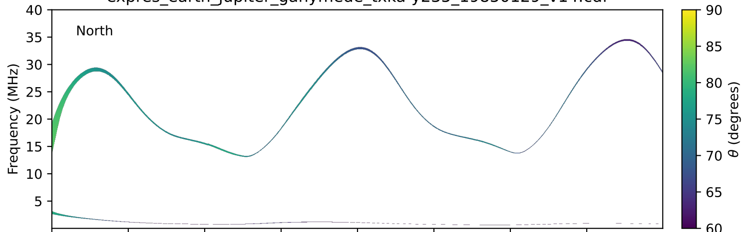
expres_earth_jupiter_ganymede_txka-y235_19850129_v14.cdf
