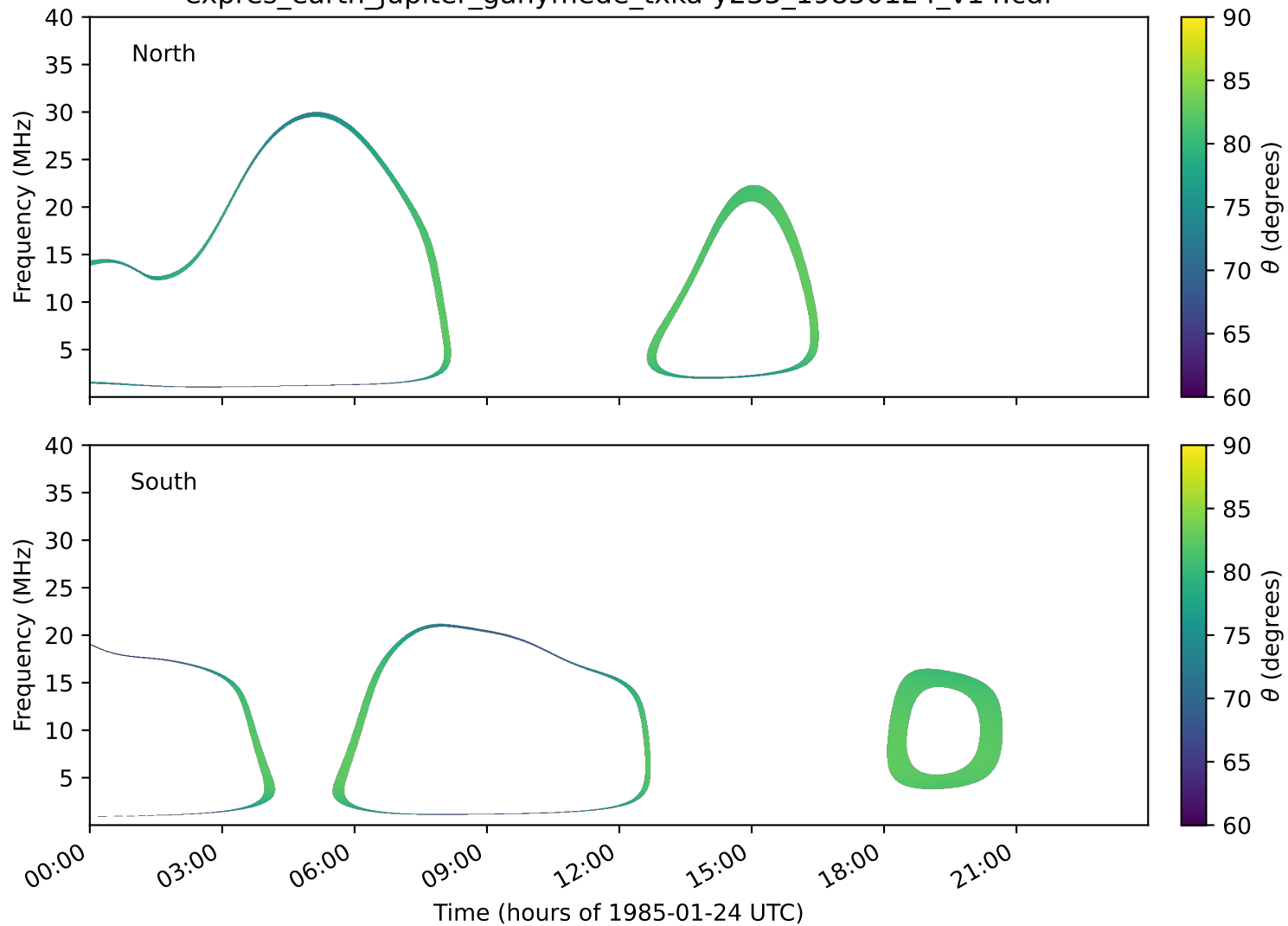
expres_earth_jupiter_ganymede_txka-y235_19850124_v14.cdf
