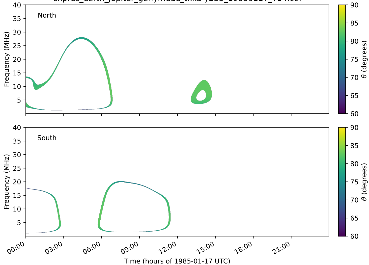
expres_earth_jupiter_ganymede_txka-y235_19850117_v14.cdf
