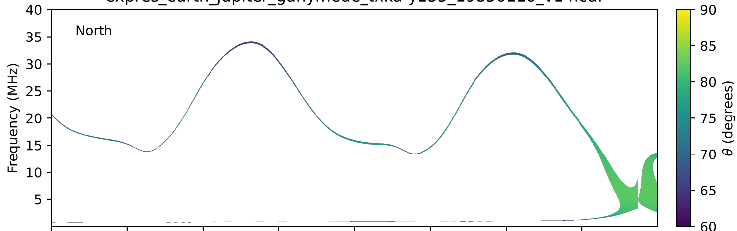
expres_earth_jupiter_ganymede_txka-y235_19850116_v14.cdf
