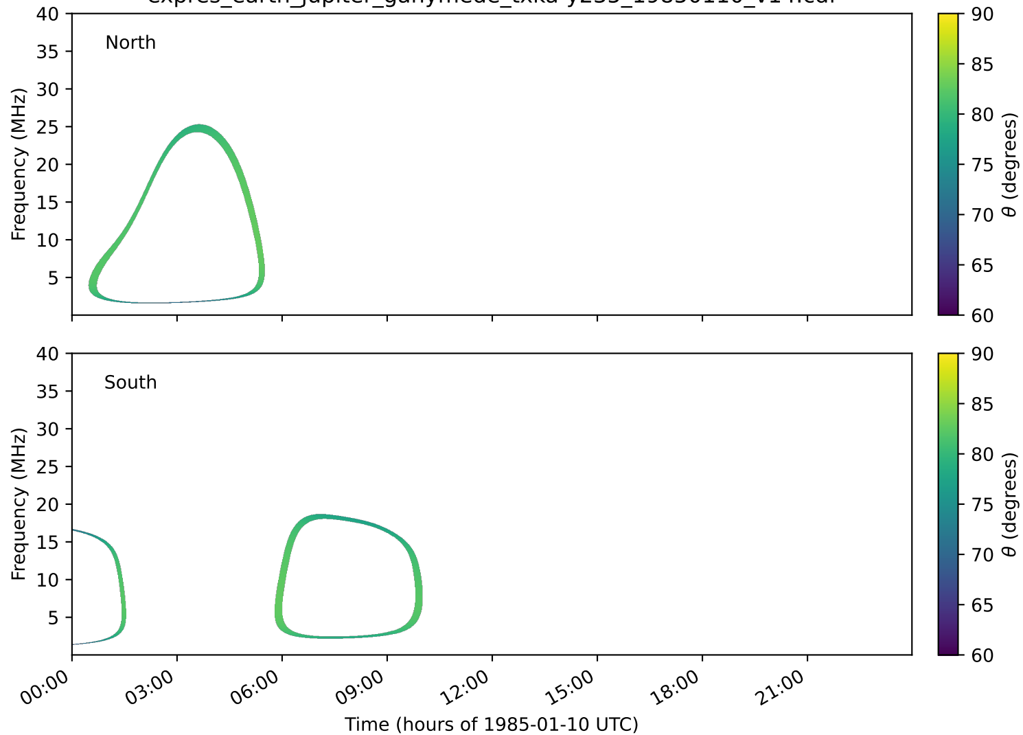
expres_earth_jupiter_ganymede_txka-y235_19850110_v14.cdf
