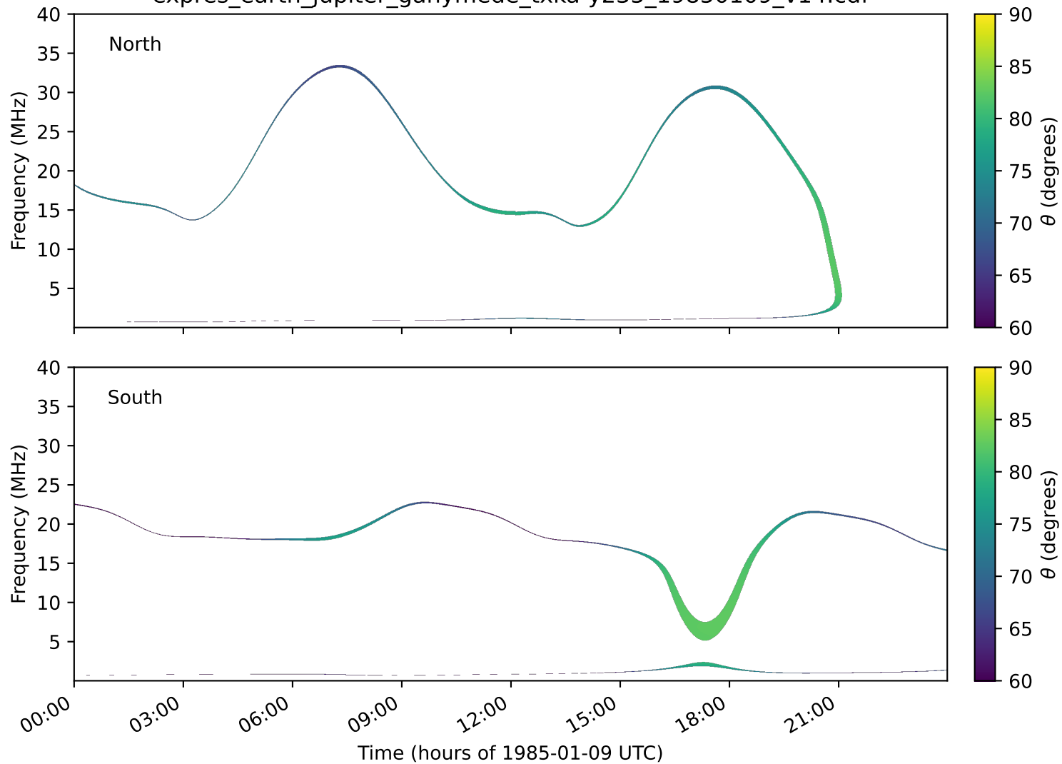
expres_earth_jupiter_ganymede_txka-y235_19850109_v14.cdf
