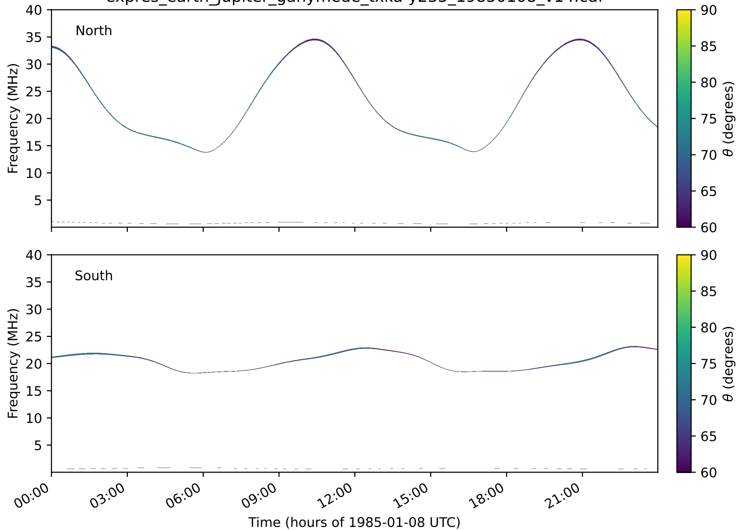
expres_earth_jupiter_ganymede_txka-y235_19850108_v14.cdf
