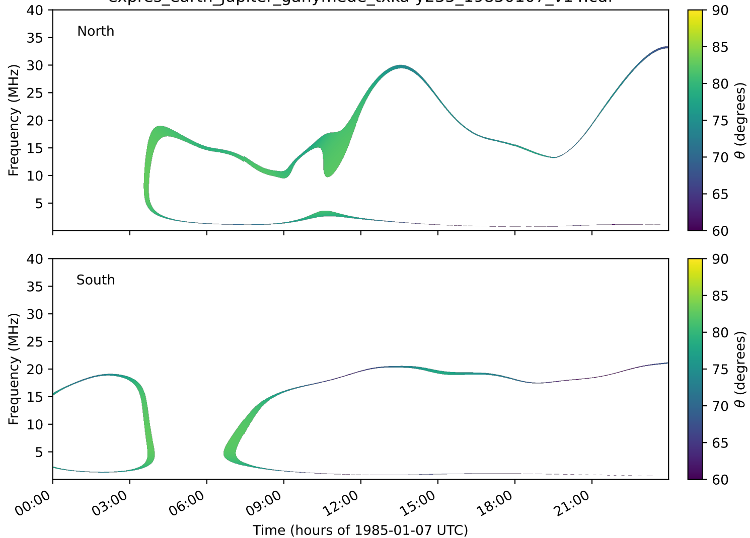
expres_earth_jupiter_ganymede_txka-y235_19850107_v14.cdf
