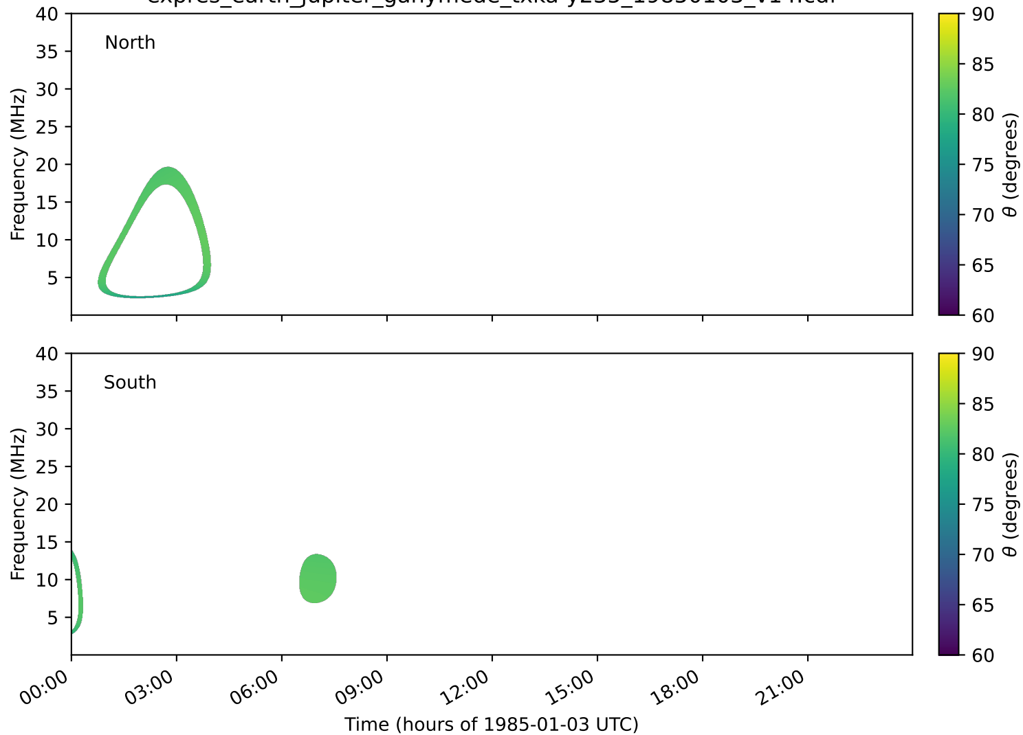
expres_earth_jupiter_ganymede_txka-y235_19850103_v14.cdf
