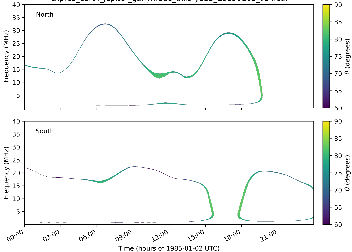
expres_earth_jupiter_ganymede_txka-y235_19850102_v14.cdf
