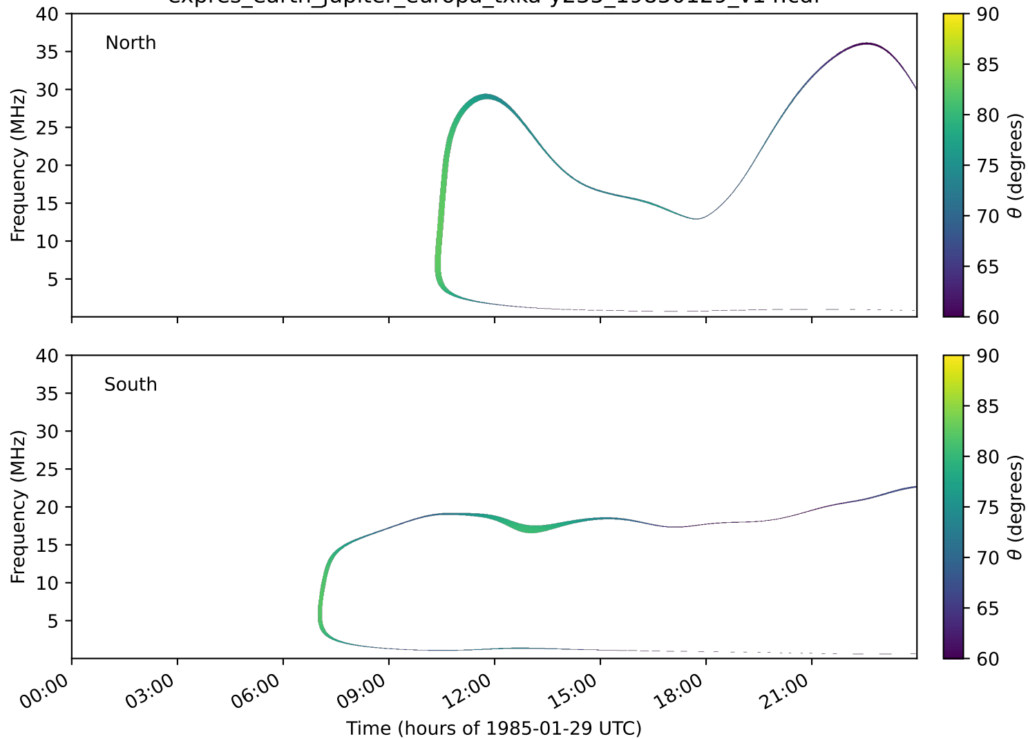
expres_earth_jupiter_europa_txka-y235_19850129_v14.cdf
