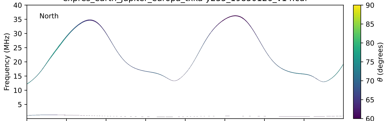
expres_earth_jupiter_europa_txka-y235_19850126_v14.cdf
