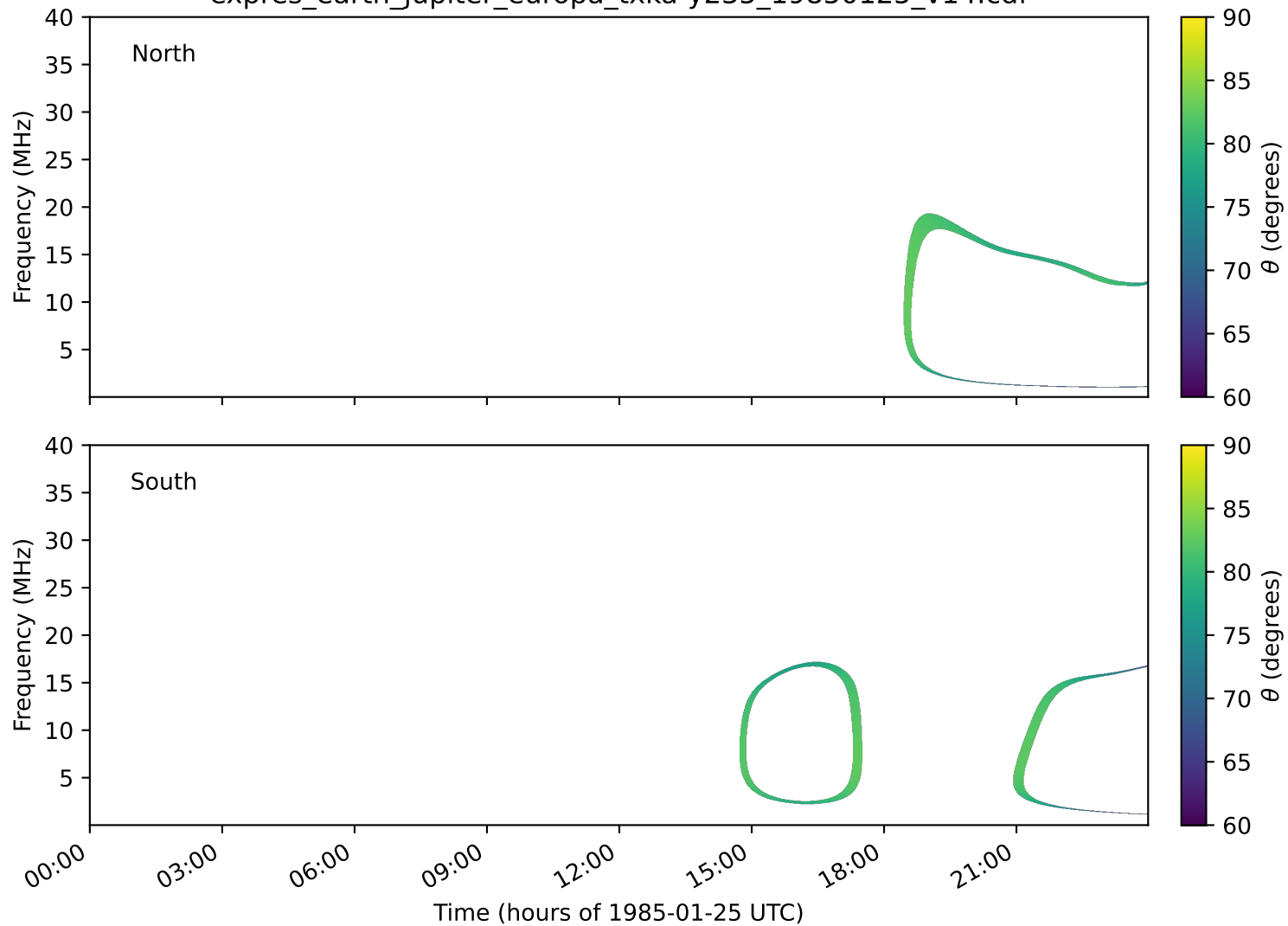
expres_earth_jupiter_europa_txka-y235_19850125_v14.cdf
