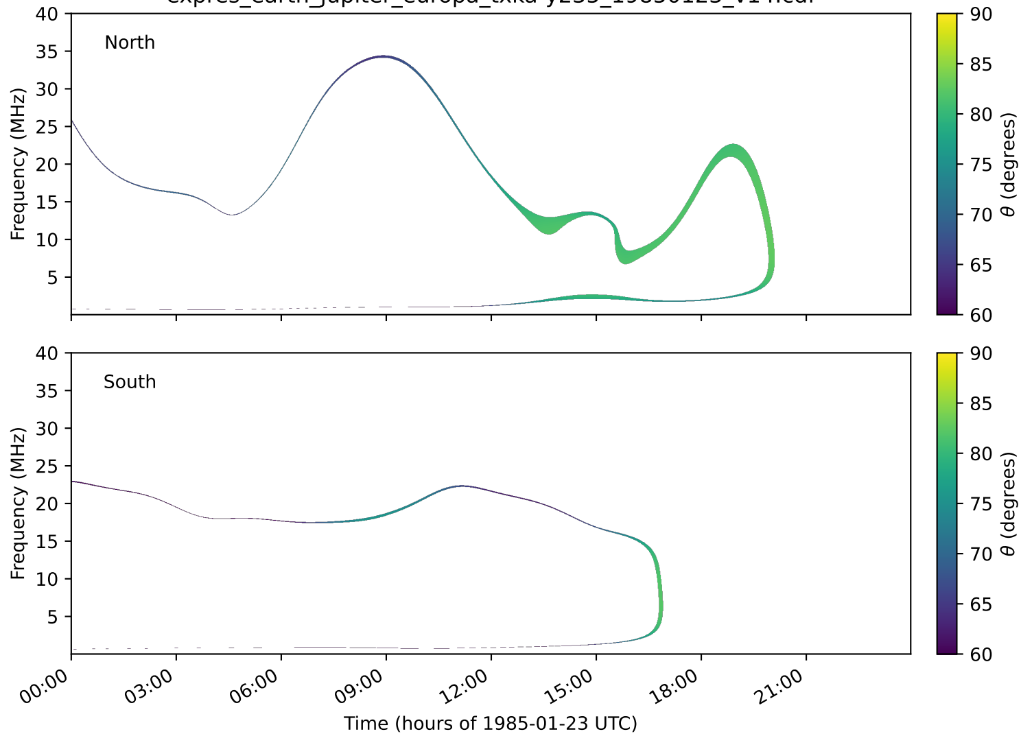
expres_earth_jupiter_europa_txka-y235_19850123_v14.cdf
