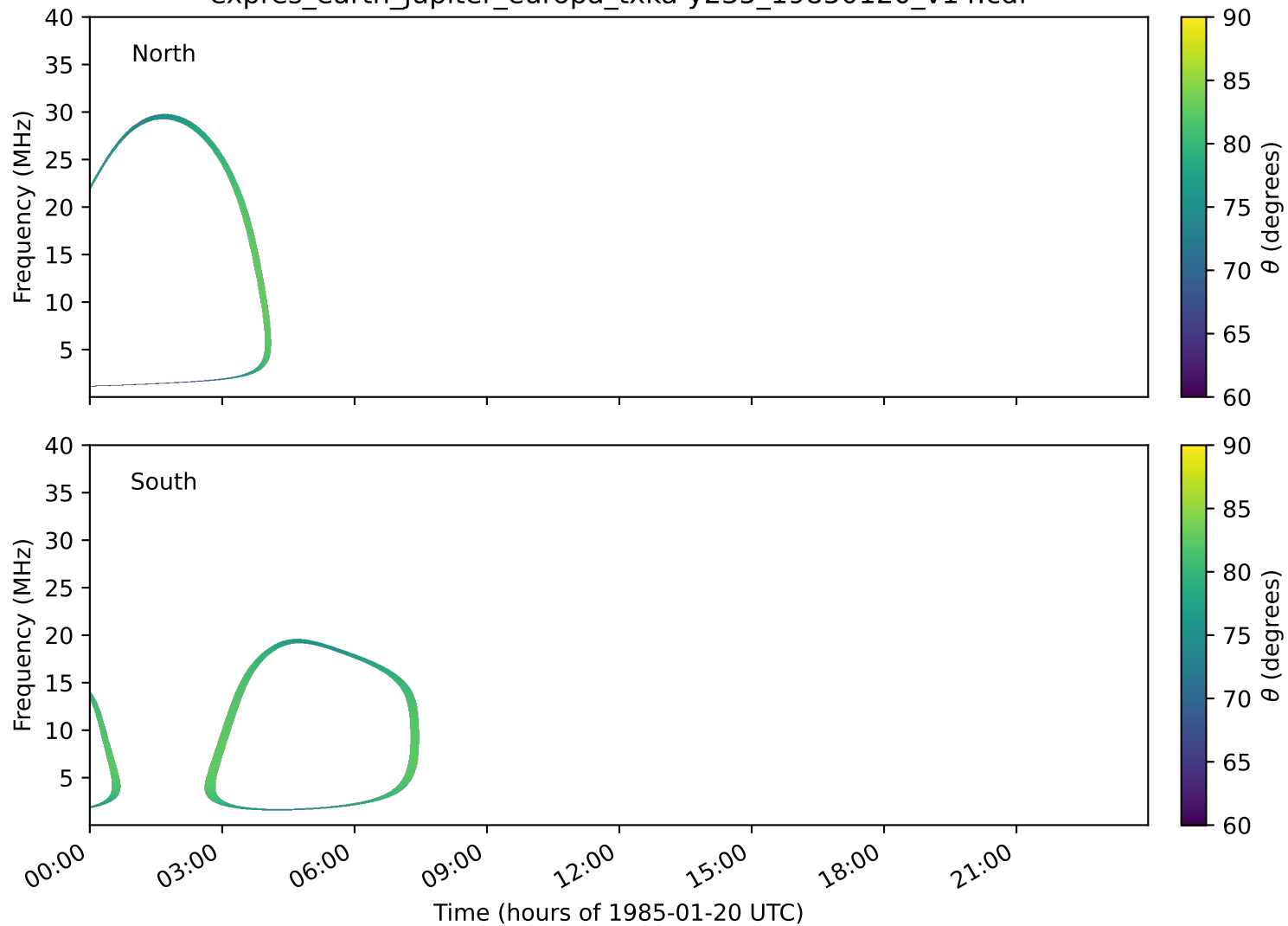
expres_earth_jupiter_europa_txka-y235_19850120_v14.cdf
