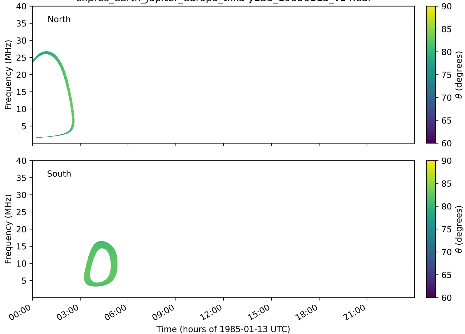
expres_earth_jupiter_europa_txka-y235_19850113_v14.cdf
