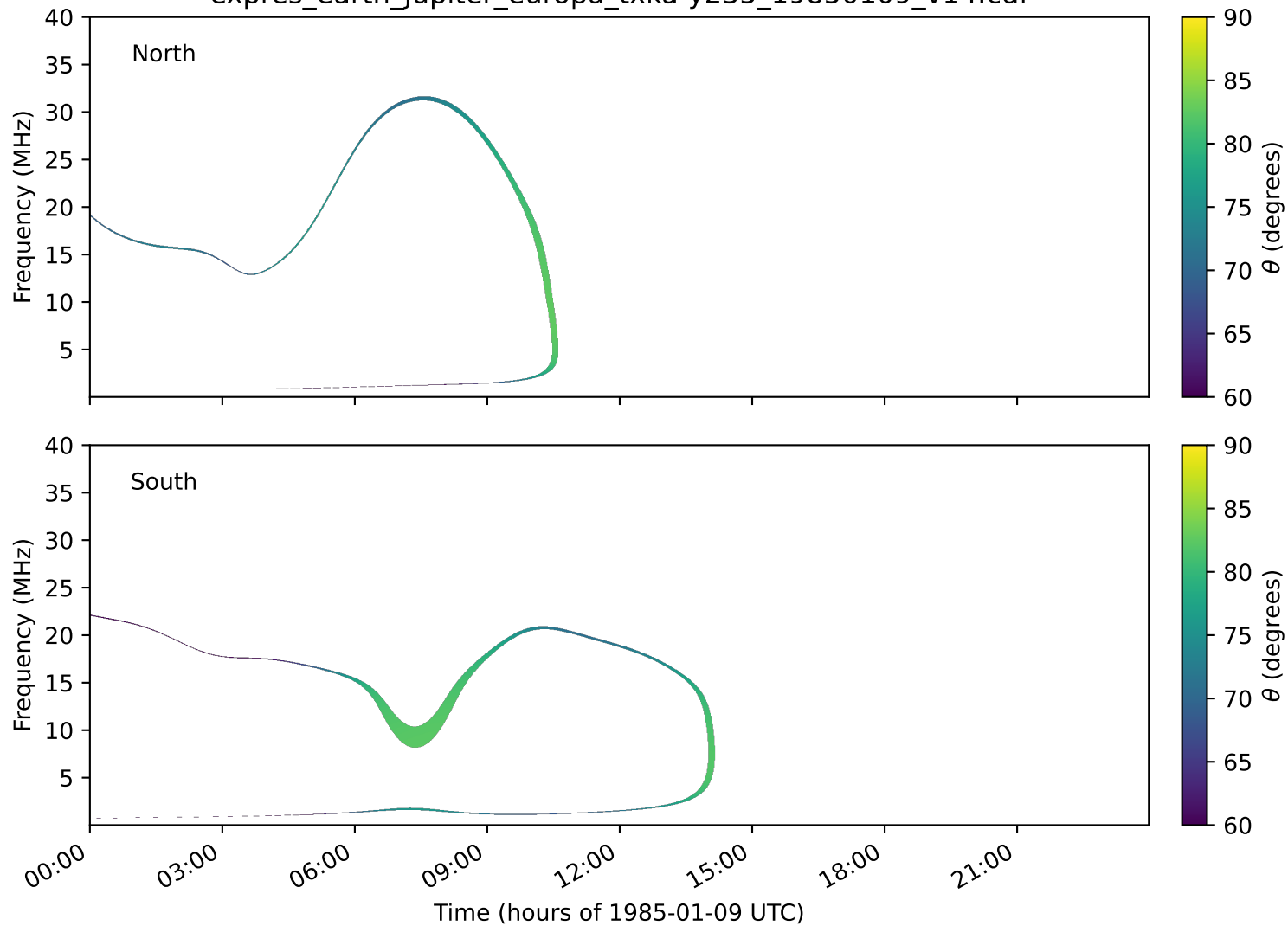
expres_earth_jupiter_europa_txka-y235_19850109_v14.cdf
