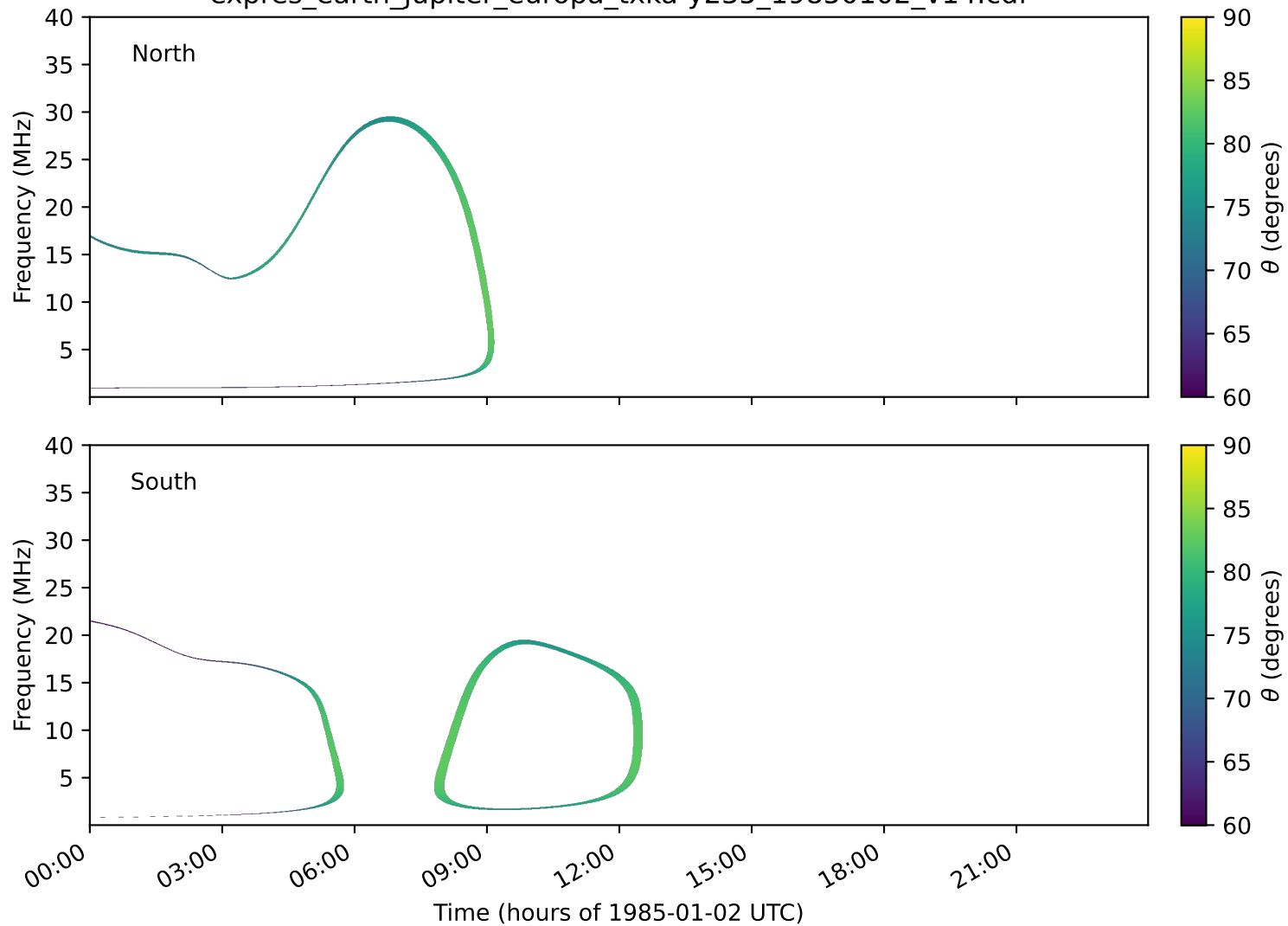
expres_earth_jupiter_europa_txka-y235_19850102_v14.cdf
