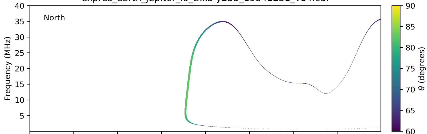
expres_earth_jupiter_io_txka-y235_19841231_v14.cdf
