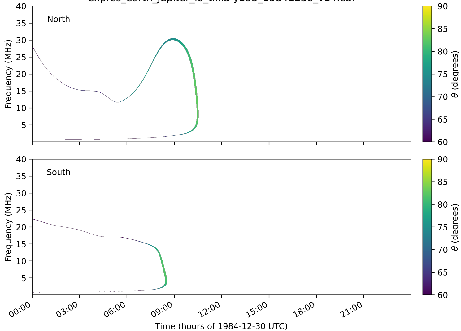
expres_earth_jupiter_io_txka-y235_19841230_v14.cdf
