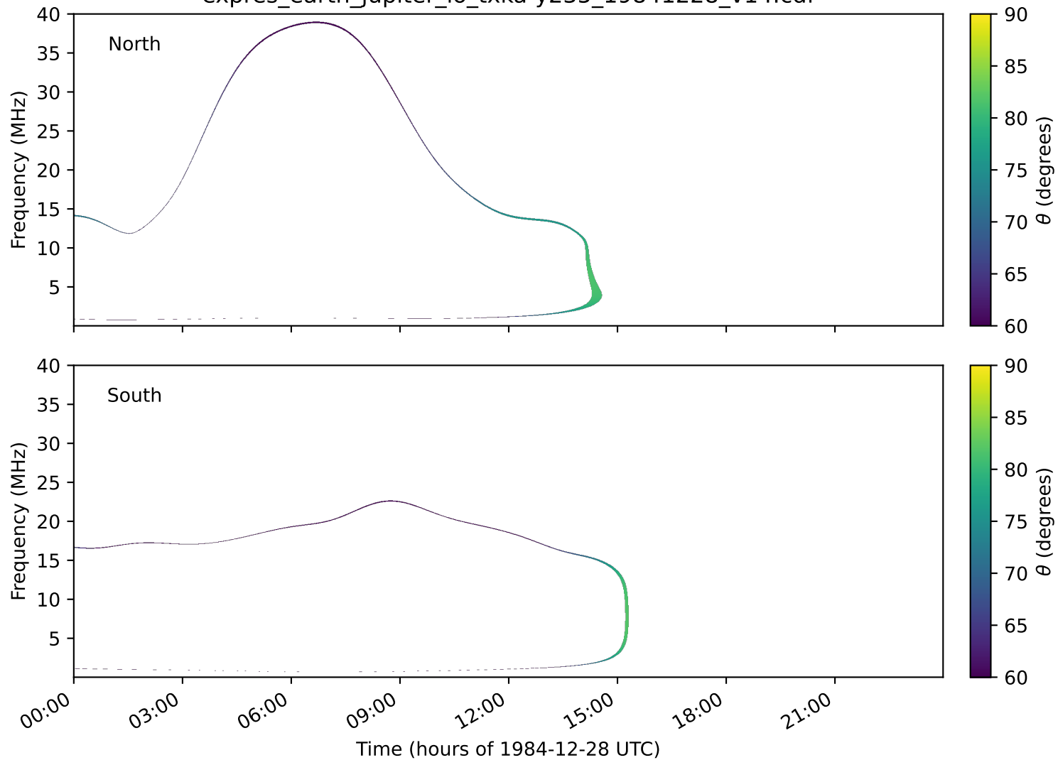
expres_earth_jupiter_io_txka-y235_19841228_v14.cdf
