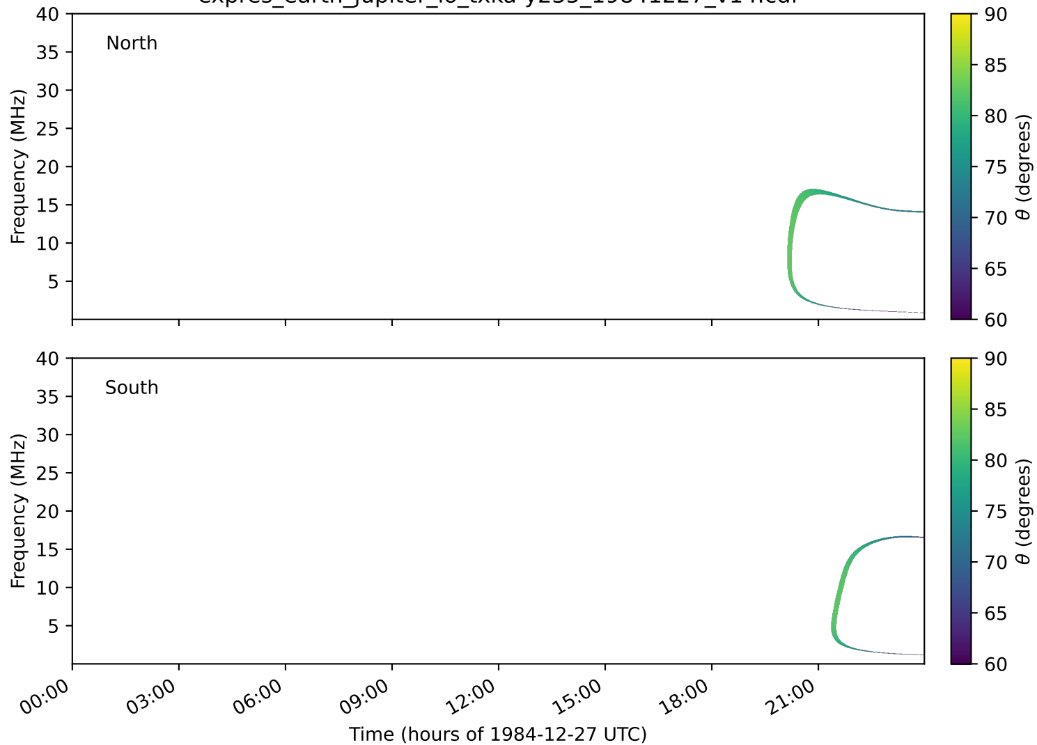
expres_earth_jupiter_io_txka-y235_19841227_v14.cdf
