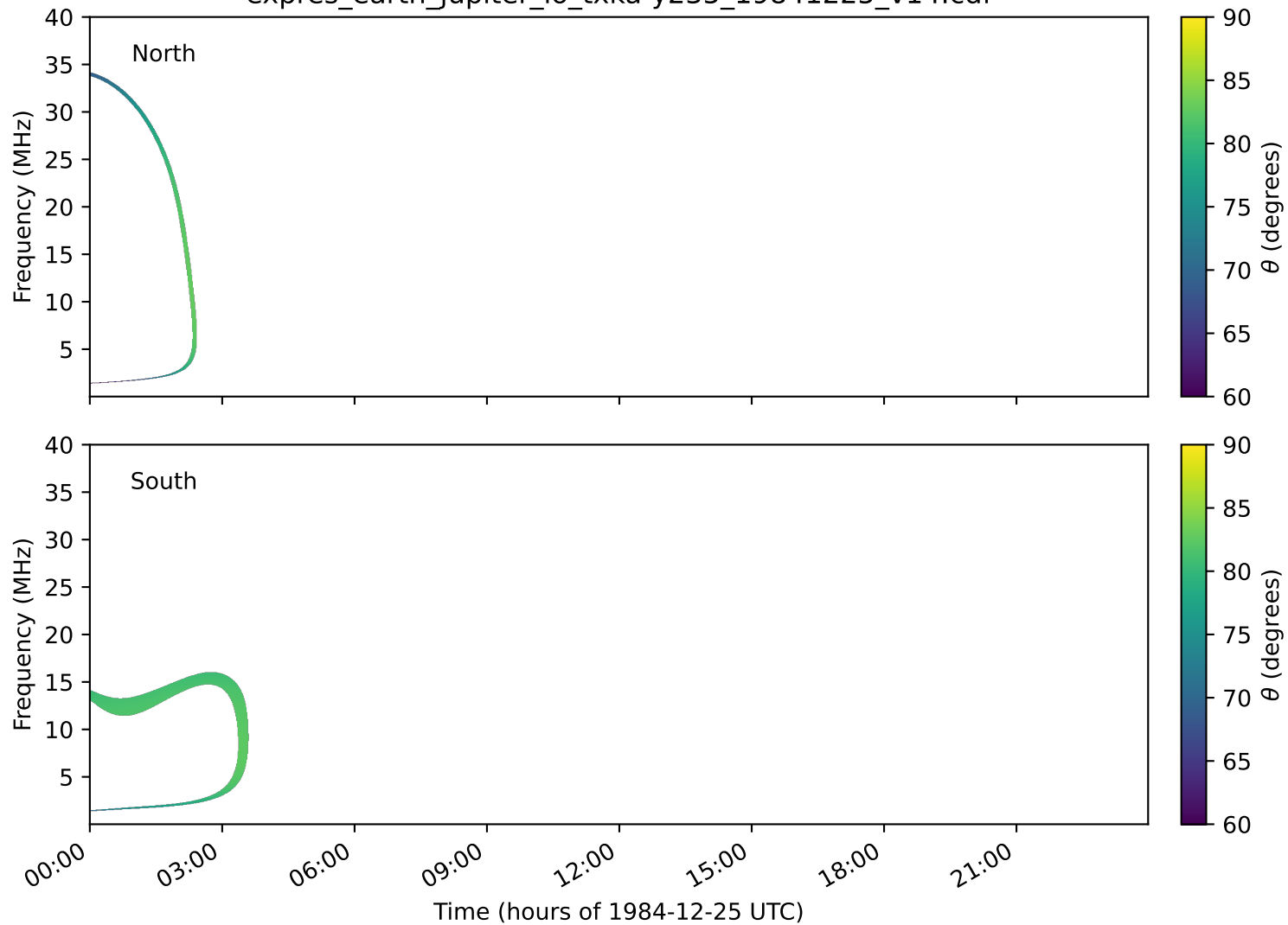
expres_earth_jupiter_io_txka-y235_19841225_v14.cdf
