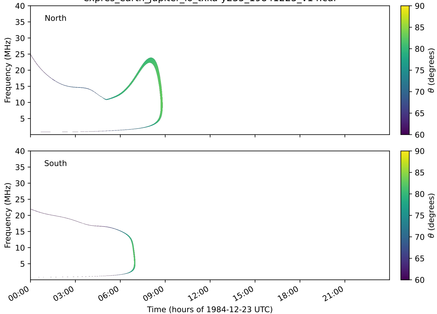
expres_earth_jupiter_io_txka-y235_19841223_v14.cdf
