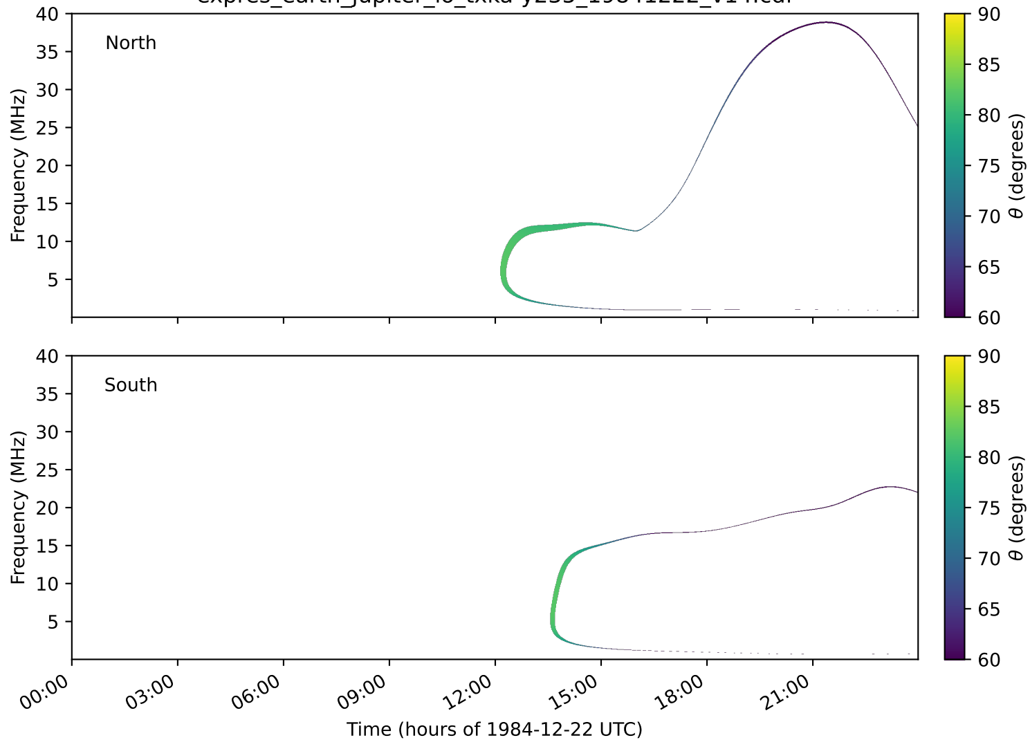
expres_earth_jupiter_io_txka-y235_19841222_v14.cdf
