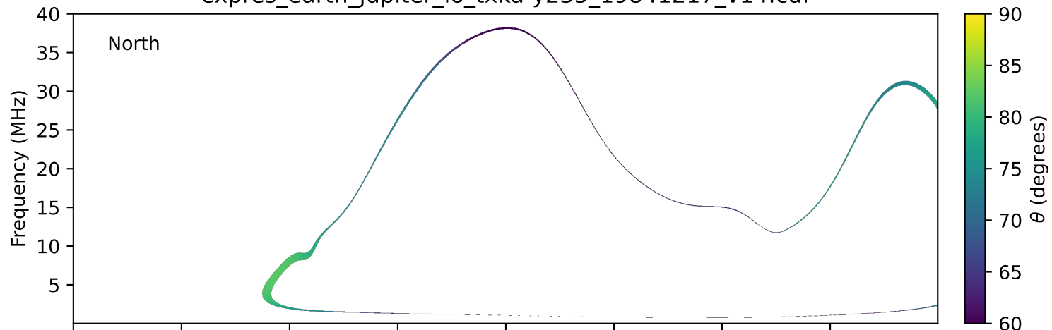
expres_earth_jupiter_io_txka-y235_19841217_v14.cdf
