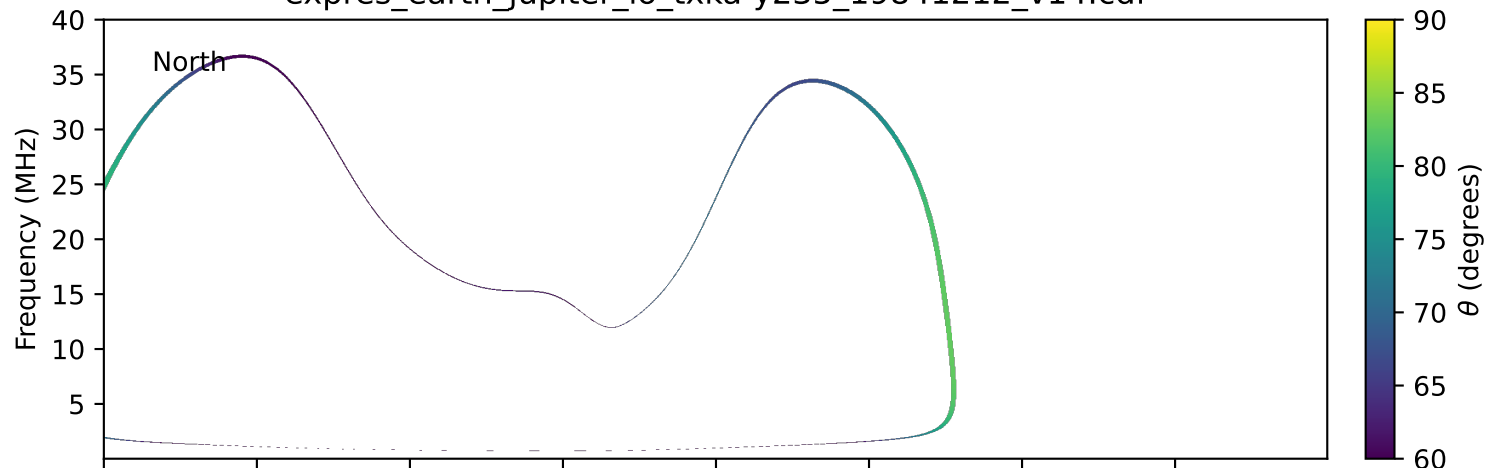
expres_earth_jupiter_io_txka-y235_19841212_v14.cdf
