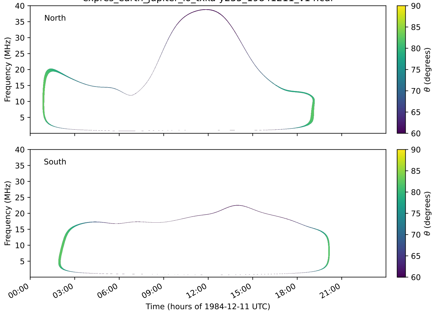
expres_earth_jupiter_io_txka-y235_19841211_v14.cdf
