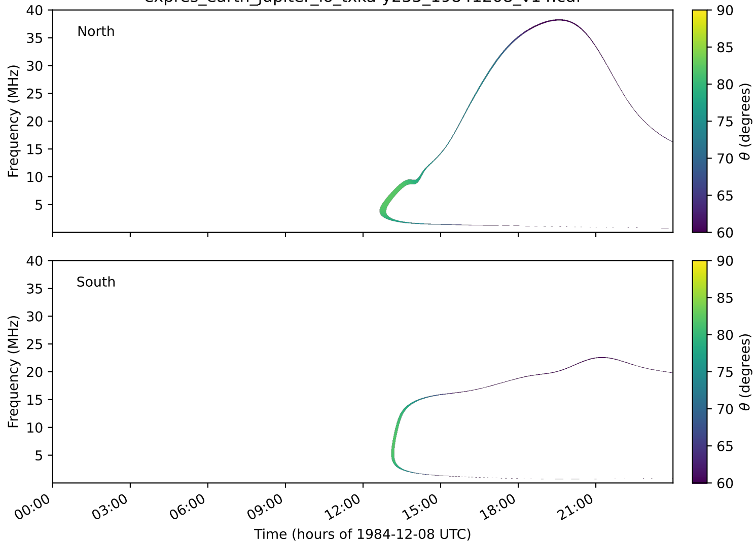
expres_earth_jupiter_io_txka-y235_19841208_v14.cdf
