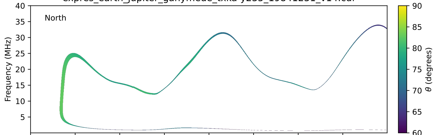
expres_earth_jupiter_ganymede_txka-y235_19841231_v14.cdf
