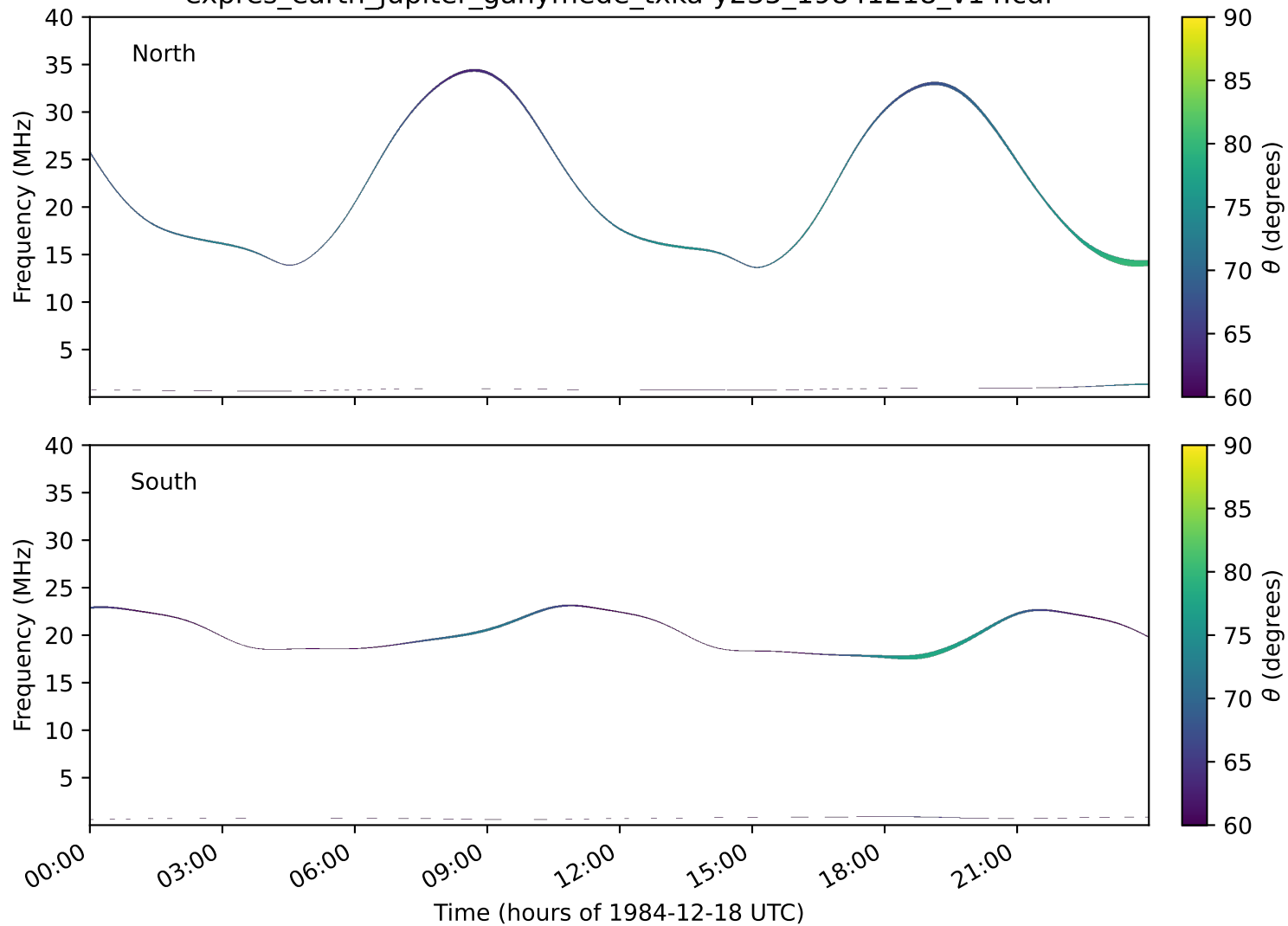
expres_earth_jupiter_ganymede_txka-y235_19841218_v14.cdf
