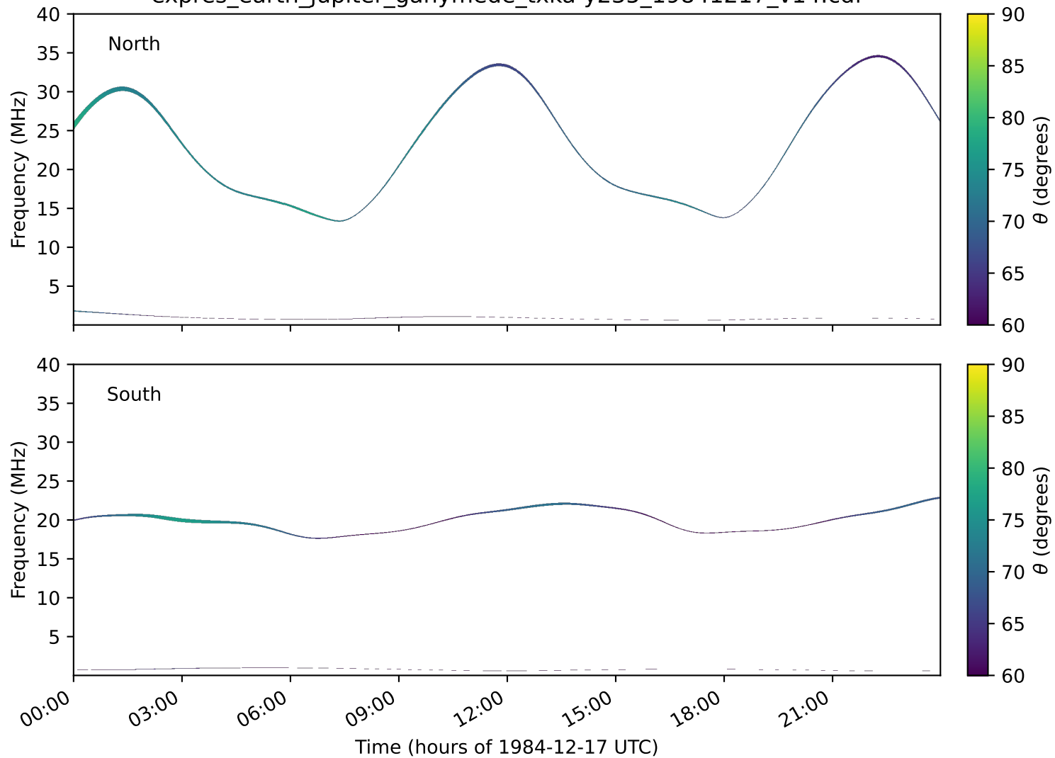
expres_earth_jupiter_ganymede_txka-y235_19841217_v14.cdf
