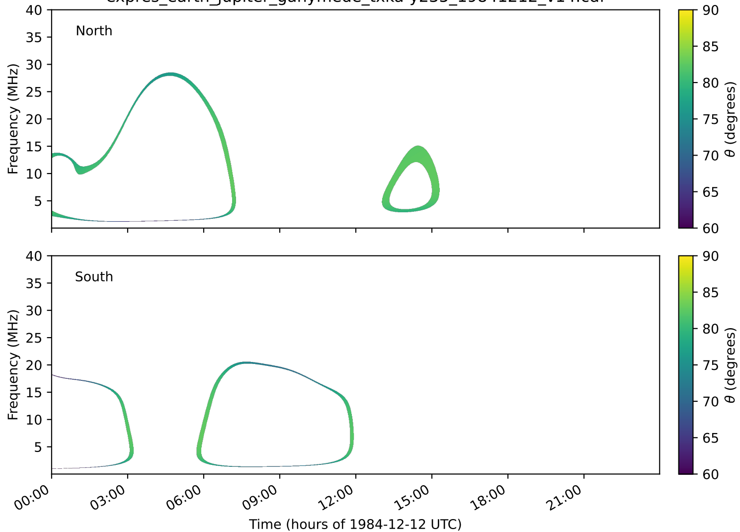
expres_earth_jupiter_ganymede_txka-y235_19841212_v14.cdf
